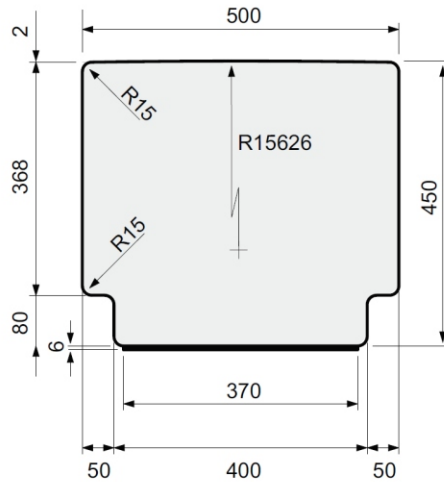
PROFILE
